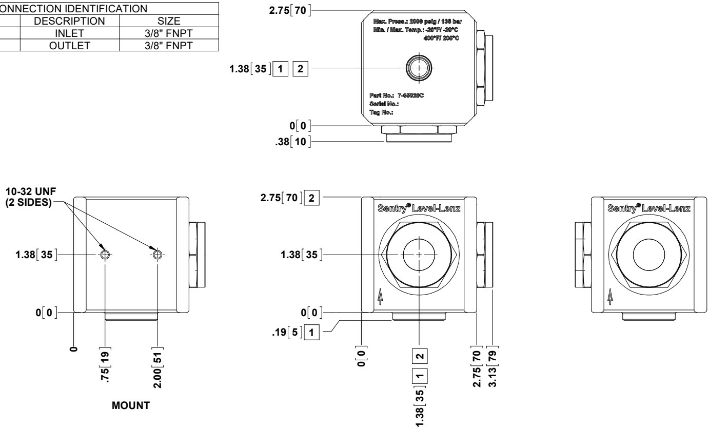
Figure 1. Sentry Level-Lenz Dimensional Drawing
